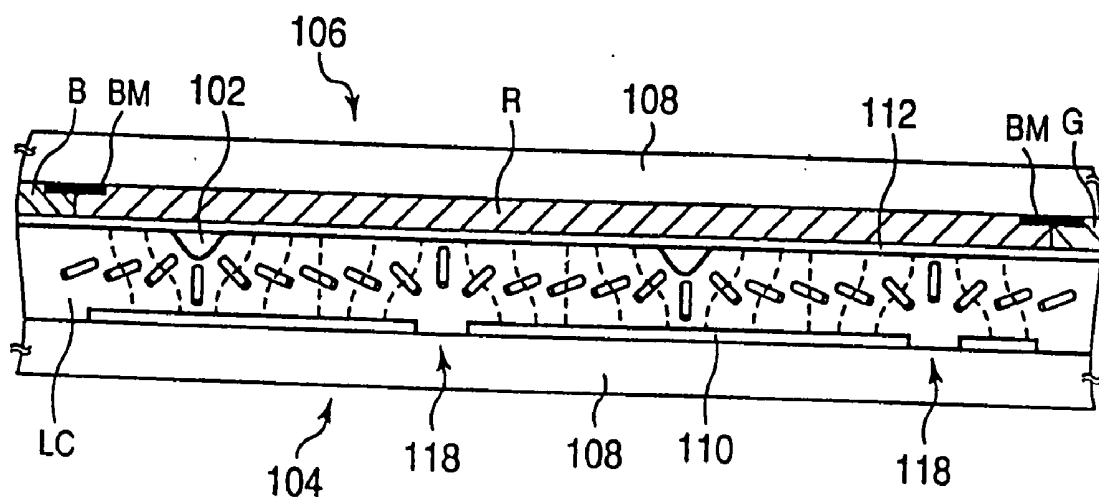
PRIOR ART FIG.39
