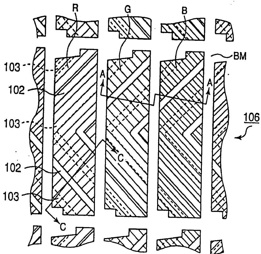
PRIOR ART FIG.35
