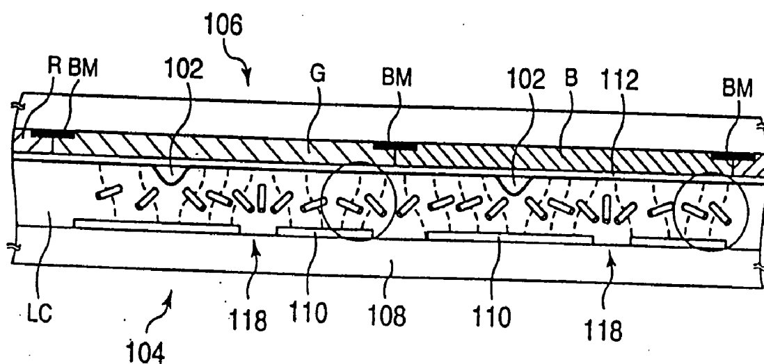
PRIOR ART FIG.40
