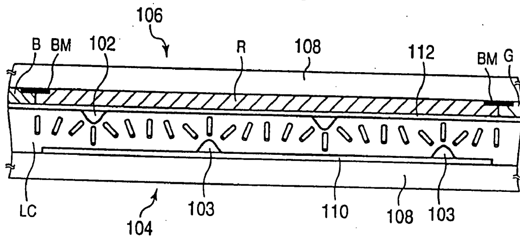
PRIOR ART FIG.37
