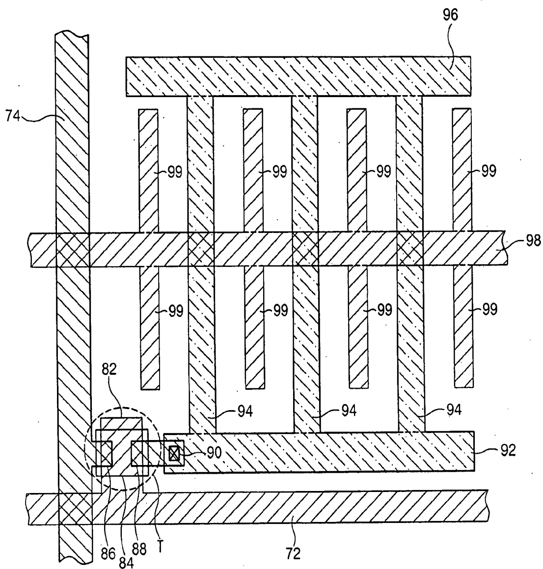
FIG. 3 (RELATED ART)
