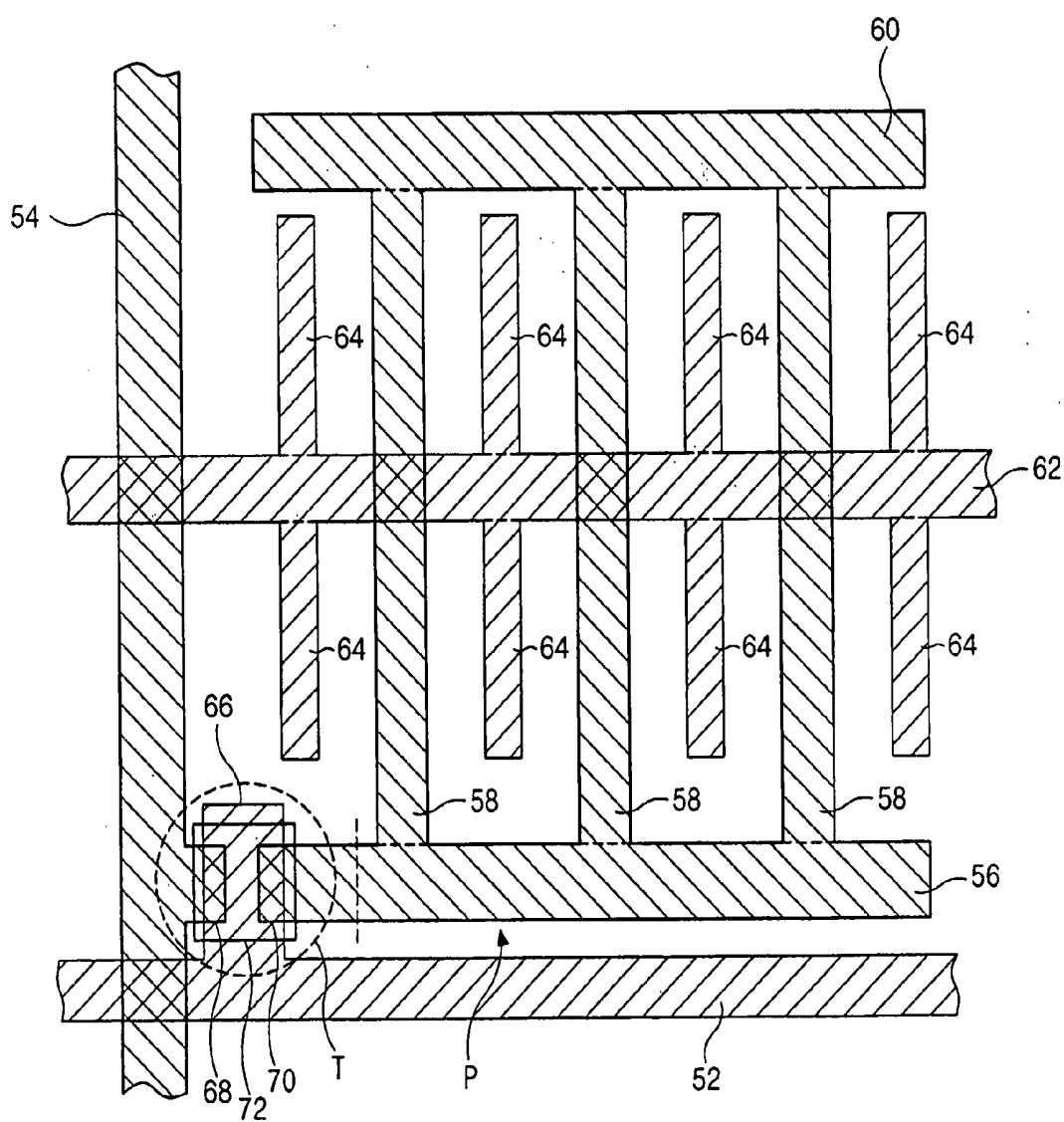
FIG. 2 (RELATED ART)
