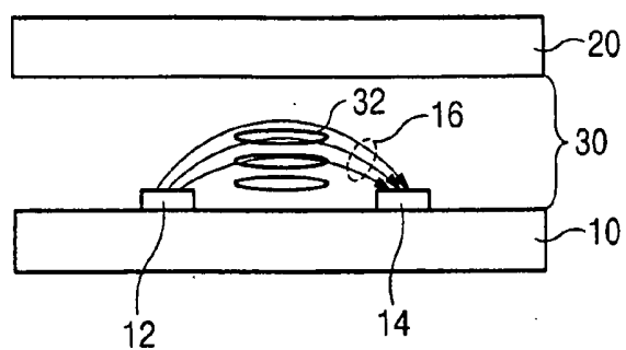
FIG. 1 (RELATED ART)
