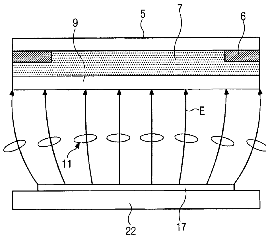
FIG. 2 RELATED ART
