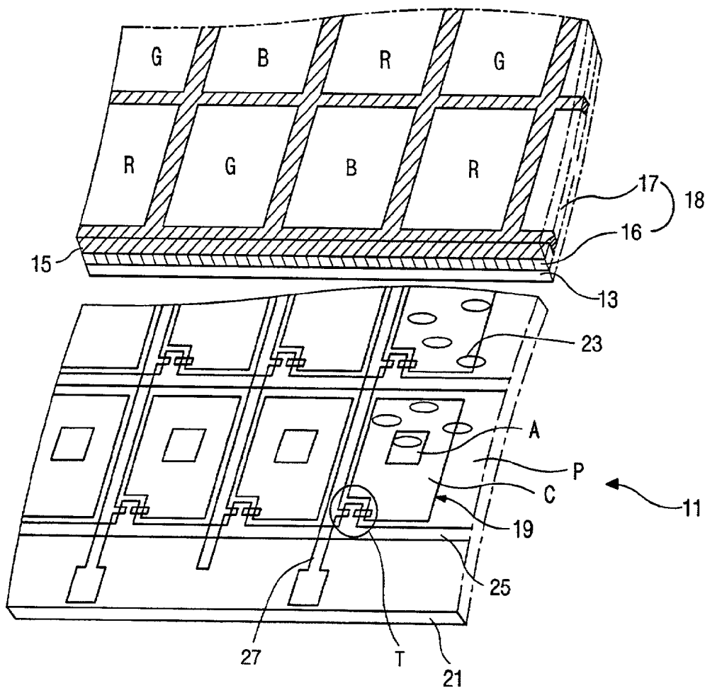
FIG. 1 (CONVENTIONAL ART)
