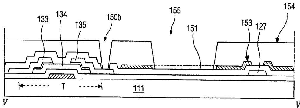
FIG. 11D
