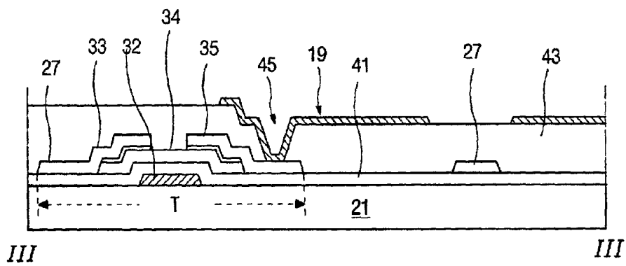
FIG. 3 (CONVENTIONAL ART)
