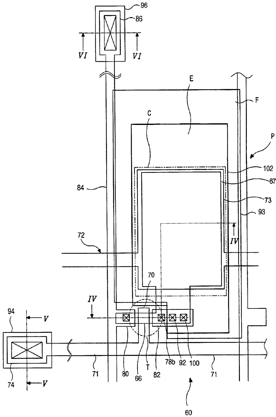
FIG. 6 (CONVENTIONAL ART)
