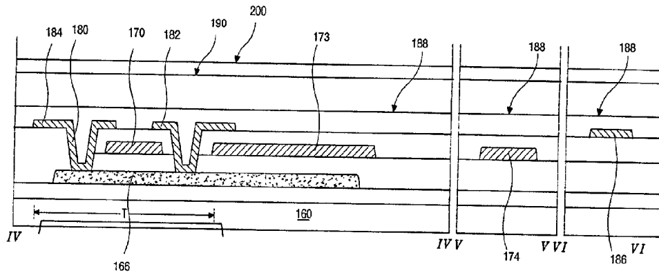
FIG. 13D
