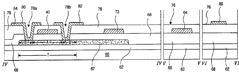
FIG. 7C (CONVENTIONAL ART)
