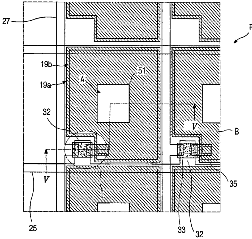
FIG. 4 (CONVENTIONAL ART)
