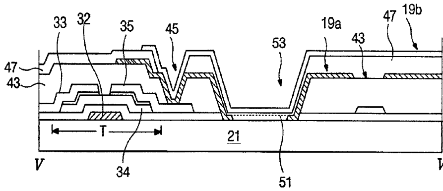
FIG. 5 (CONVENTIONAL ART)
