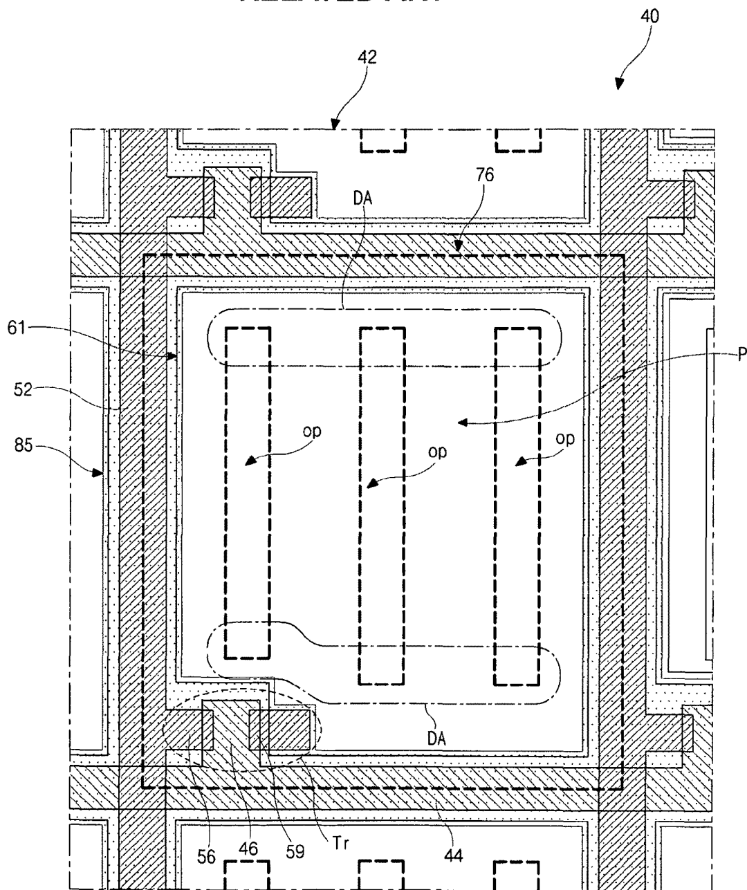
FIG. 5 RELATED ART
