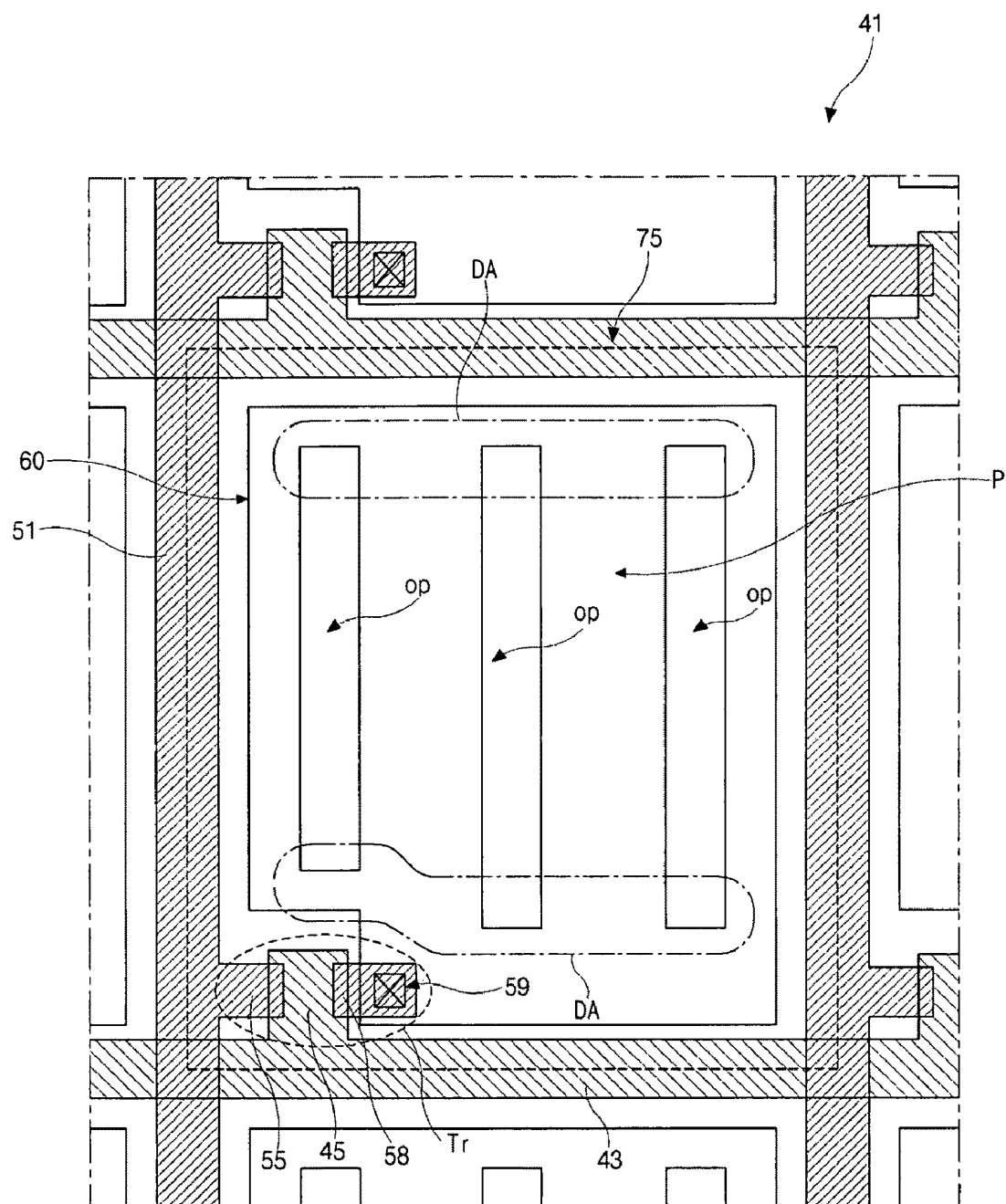
FIG. 3 RELATED ART
