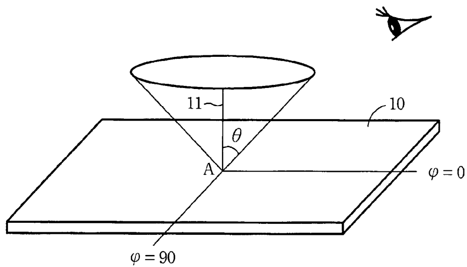
FIG. 1 (Related Art)
