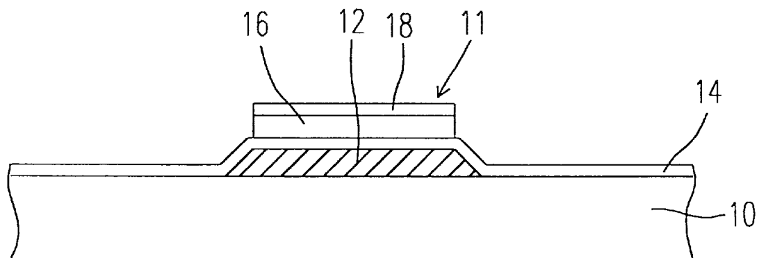
Fig. 1C(PRIOR ART)
