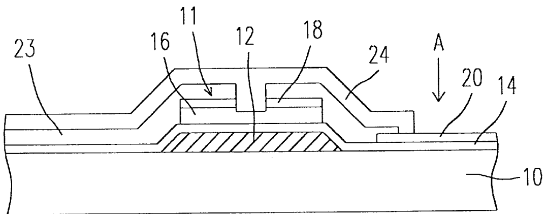
Fig. 1F(PRIOR ART)
