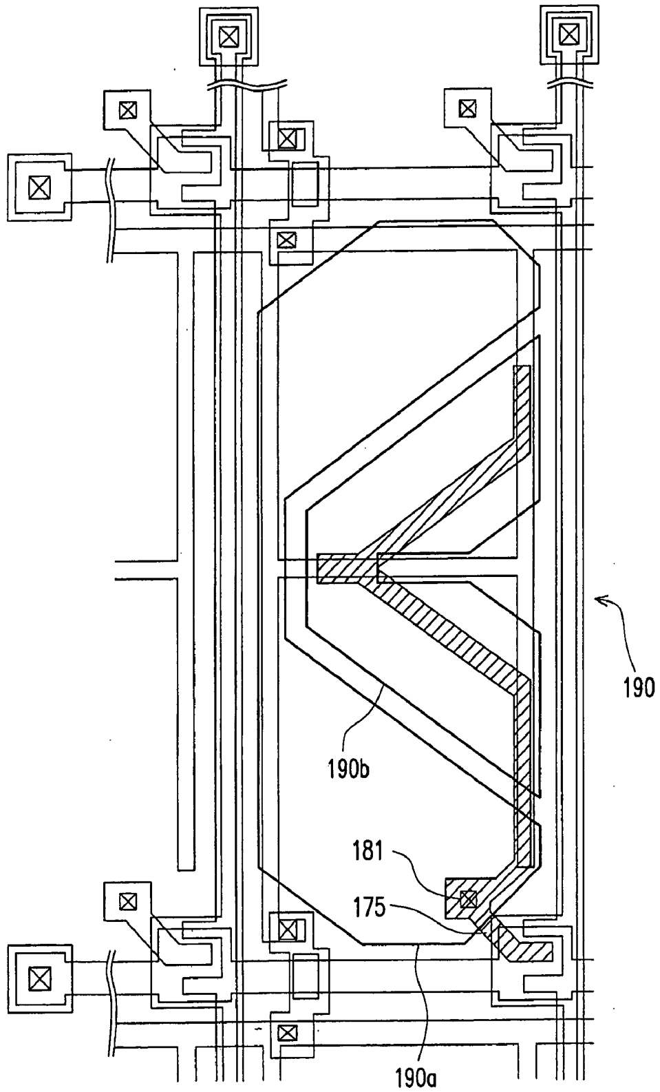
FIG. 3 (PRIOR ART)
