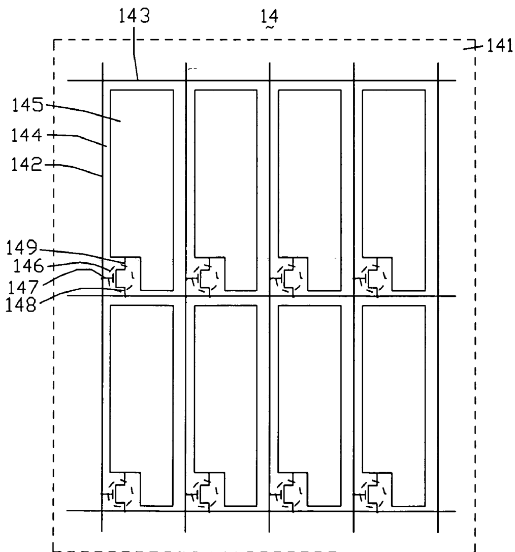
FIG. 5 (RELATED ART)
