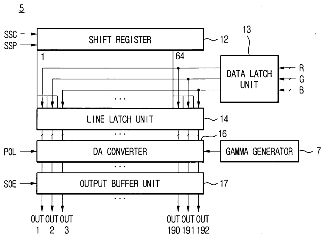
FIG. 3 (RELATED ART)
