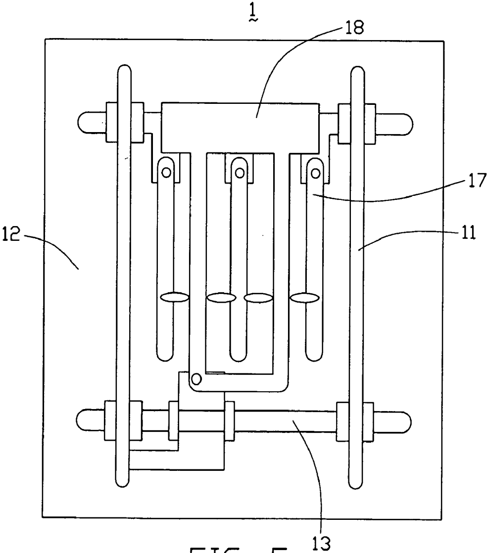
FIG. 5 (PRIOR ART)
