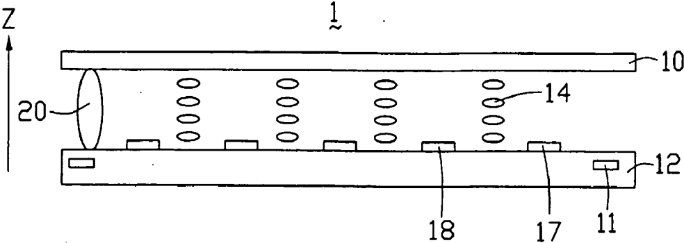
FIG. 4 (PRIOR ART)
