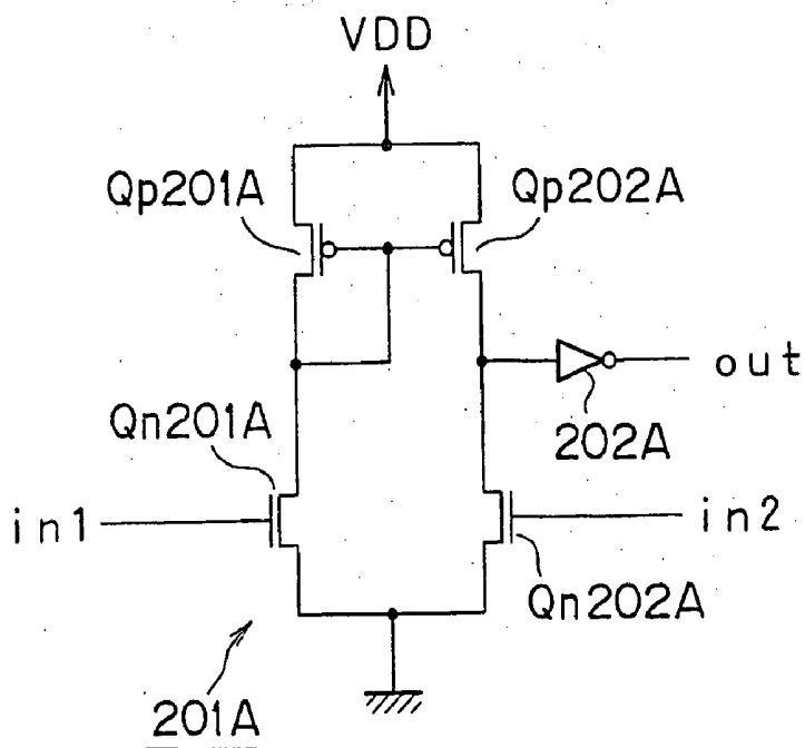
FIG. 14A RELATED ART 2
