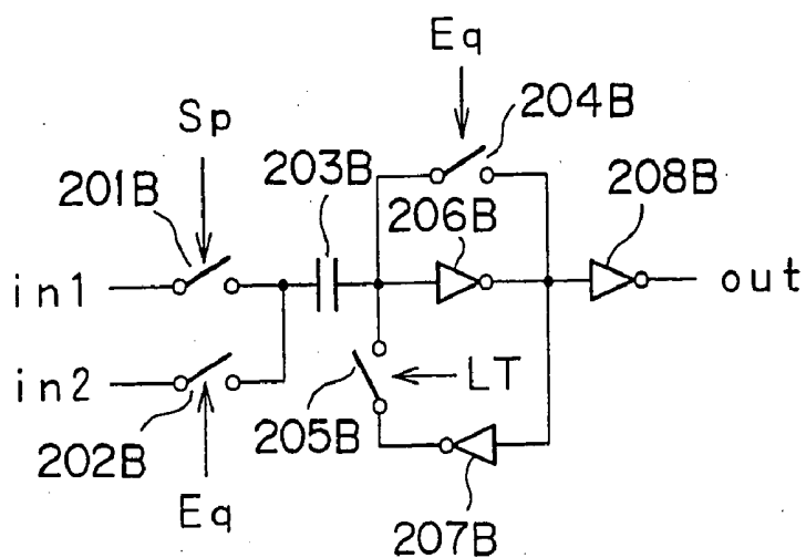
FIG. 11B RELATED ART
