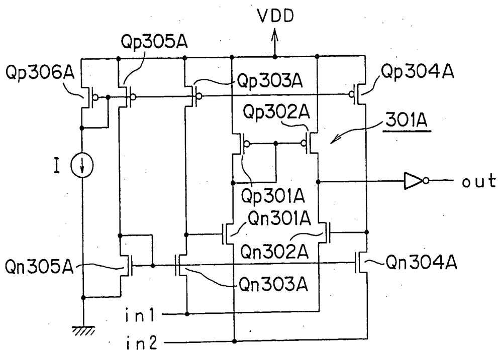
FIG. 15A RELATED ART 3
