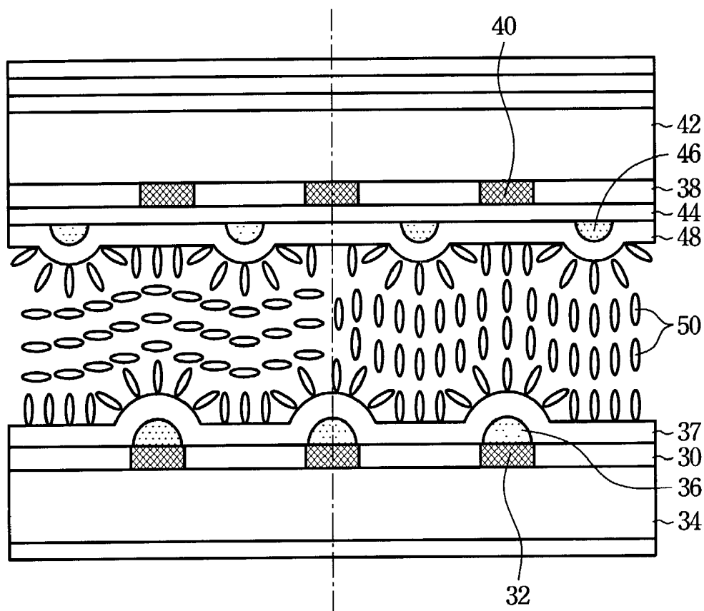
Fig. 3 (Prior Art)
