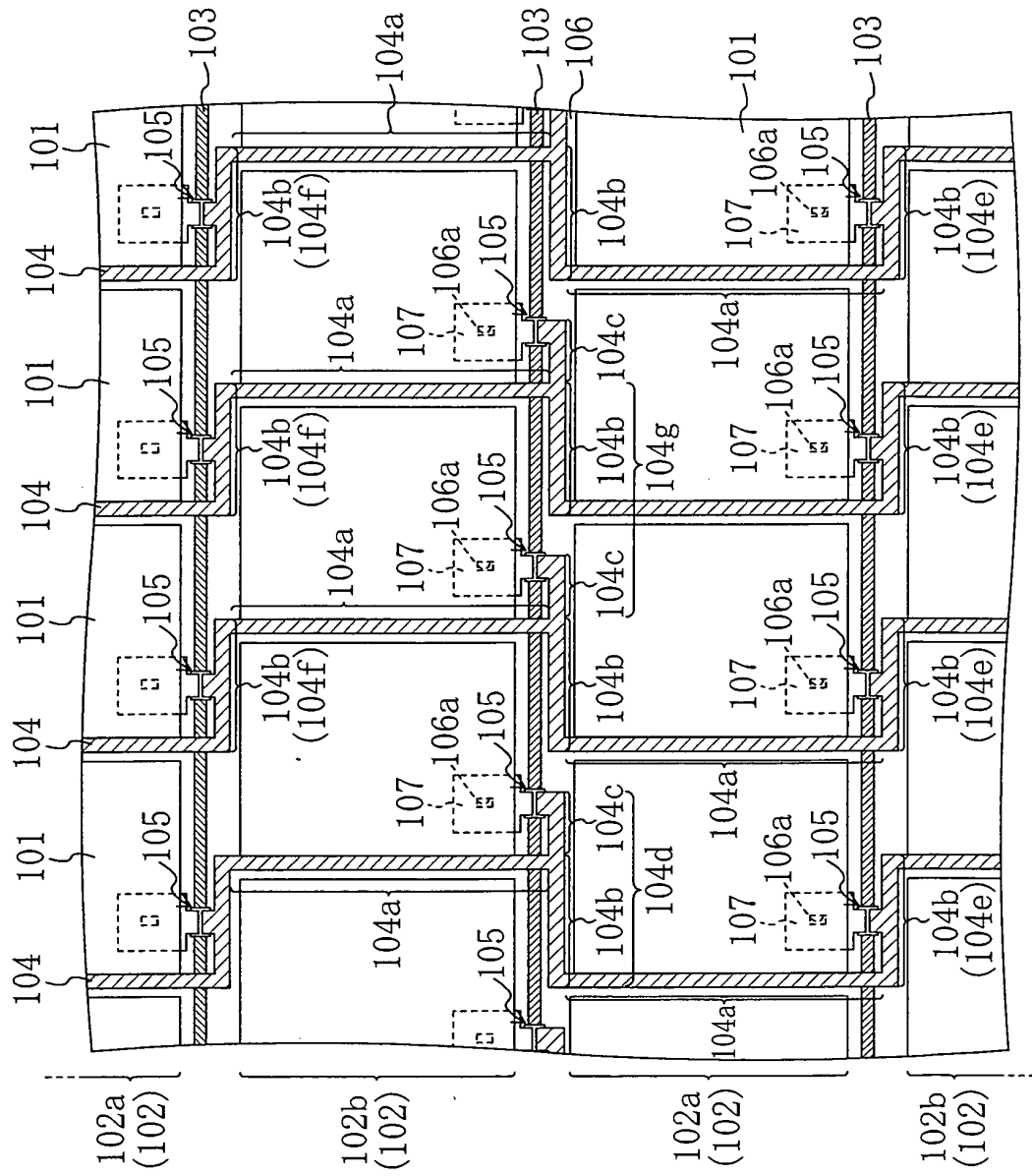
FIG. 12 PRIOR ART
