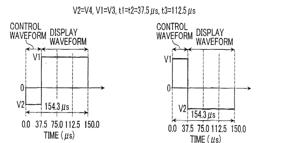
1 BIT PLANE WAVEFORM FOR DISPLAY WITH POSITIVE VOLTAGE
