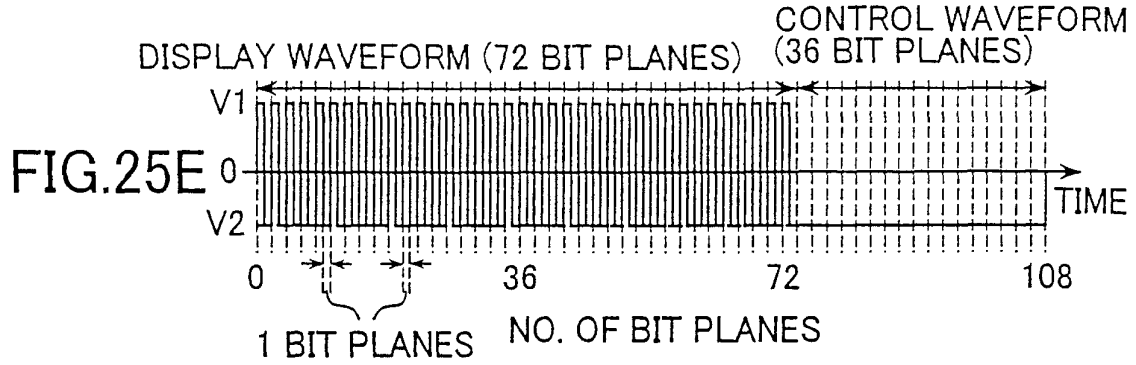
DRIVE WAVEFORM 17
