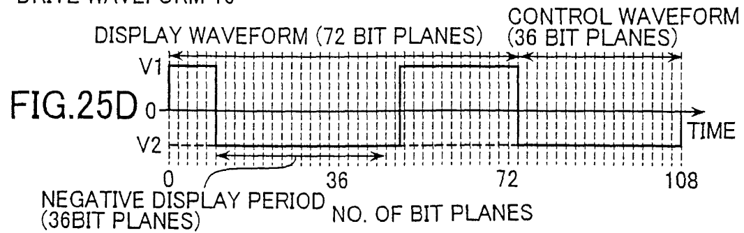
DRIVE WAVEFORM 16
