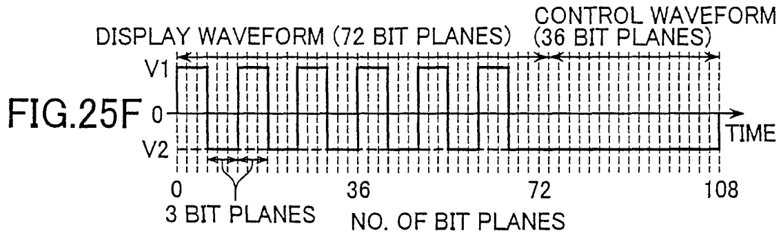
DRIVE WAVEFORM 18
