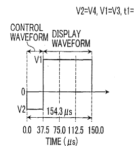
1 BIT PLANE WAVEFORM FOR DISPLAY WITH POSITIVE VOLTAGE
