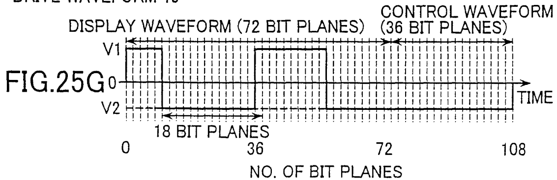
DRIVE WAVEFORM 19
