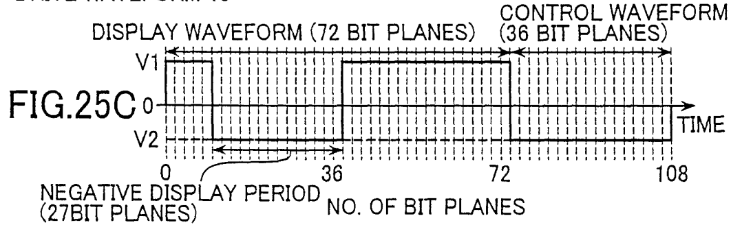
DRIVE WAVEFORM 15
