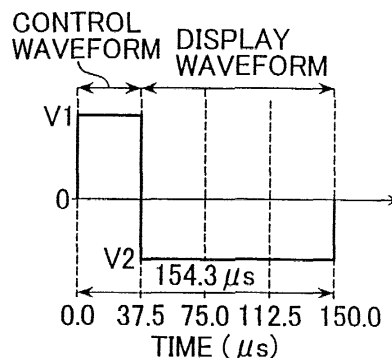
1 BIT PLANE WAVEFORM FOR DISPLAY WITH NEGATIVE VOLTAGE
