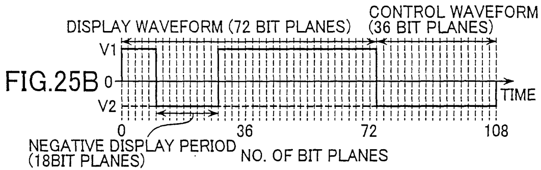
DRIVE WAVEFORM 14
