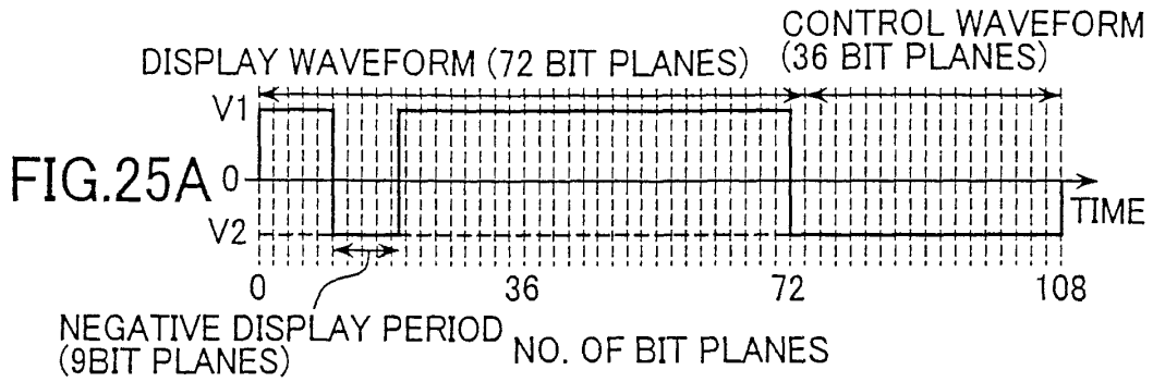
DRIVE WAVEFORM 13
