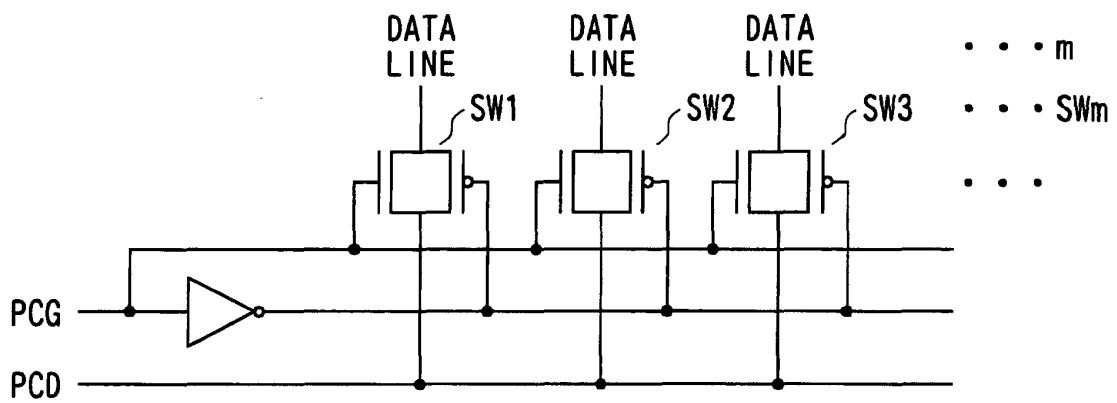
230 : PRE-CHARGE DRIVER
