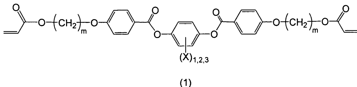
[Chemical formula 1]
