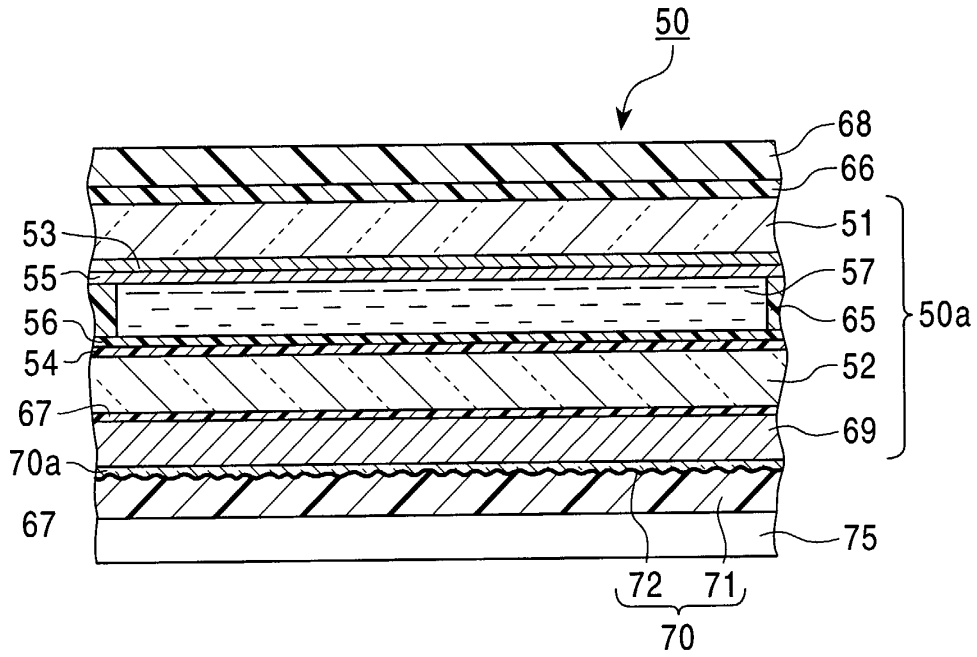
FIG. 19 PRIOR ART
