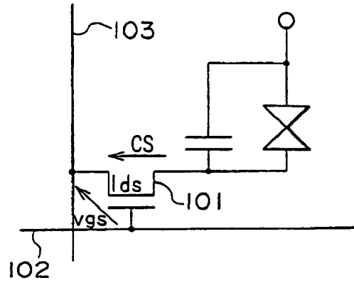
FIG. 25 RELATED ART
