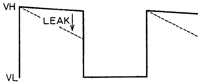
FIG. 25 RELATED ART
