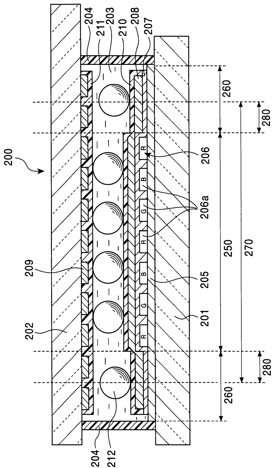
FIG. 7 PRIOR ART
