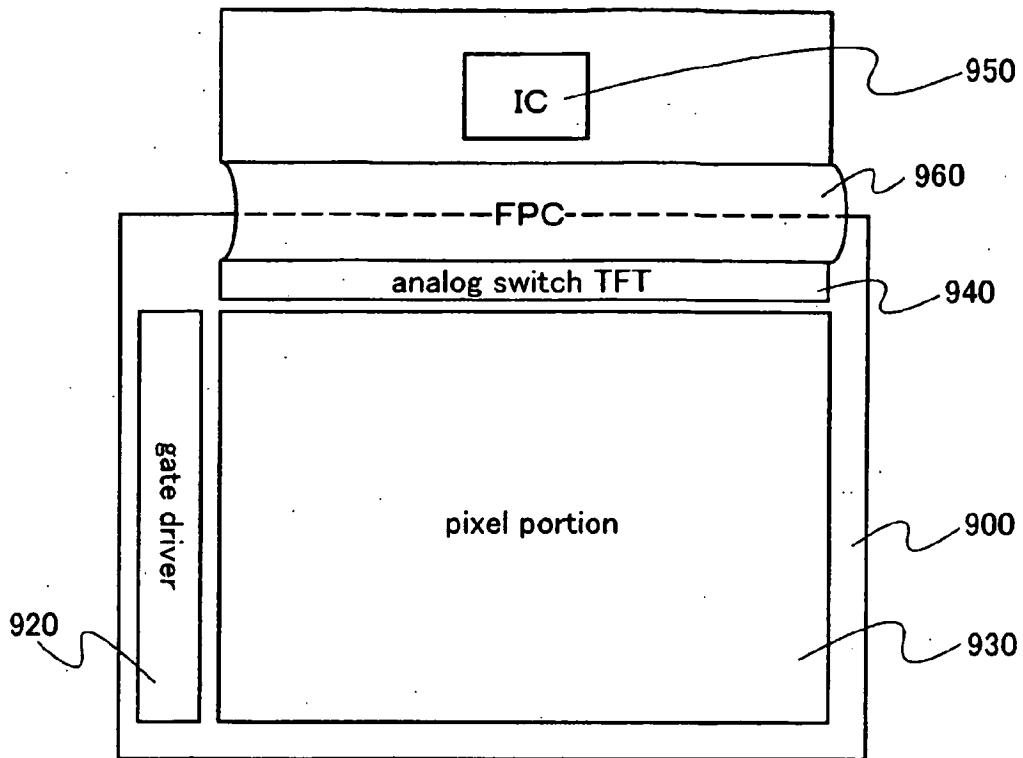
FIG. 17A IC connected by FPC
