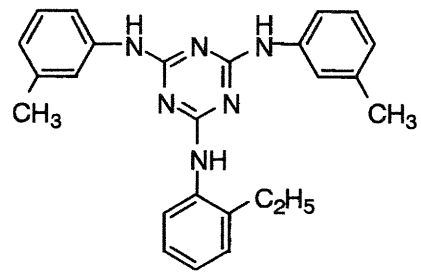
I-(10)
