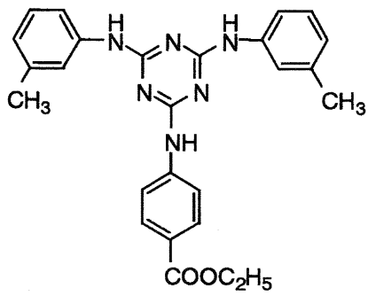
I-(11)
