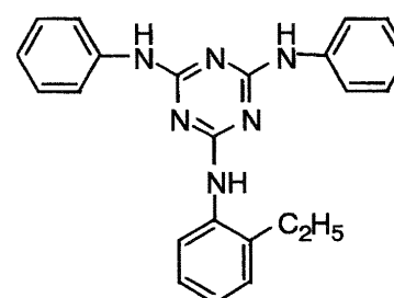
III-(8)
