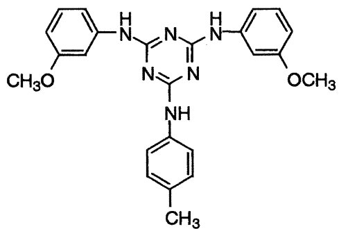
I-(39)
