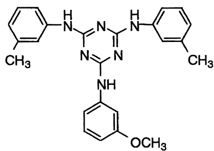
I-(7)
