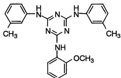
I-(7)
