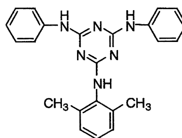
III-(4)
