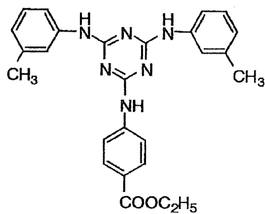
I-(11)
