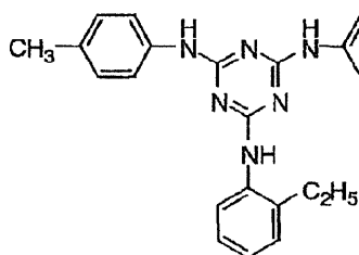
II-(5)
