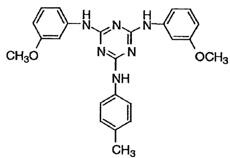
I-(39)
