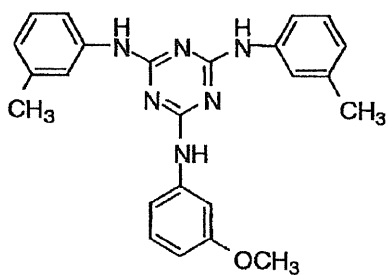
I-(7)
