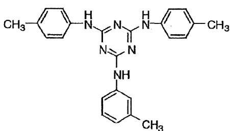
II-(4)
