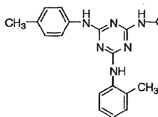
II-(3)
