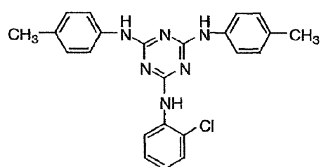
II-(4)
