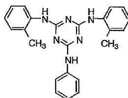
I-(50)
