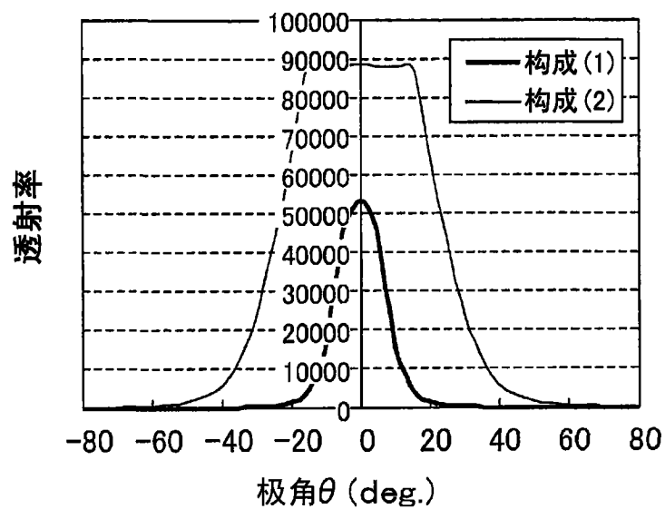
对比度视角特性[方位角: 45^\circ (550nm)]
