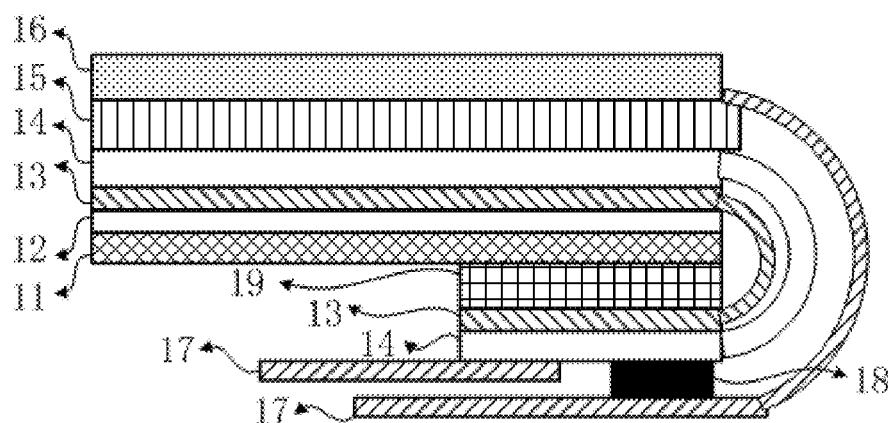
FIG. 1 (Prior Art)
